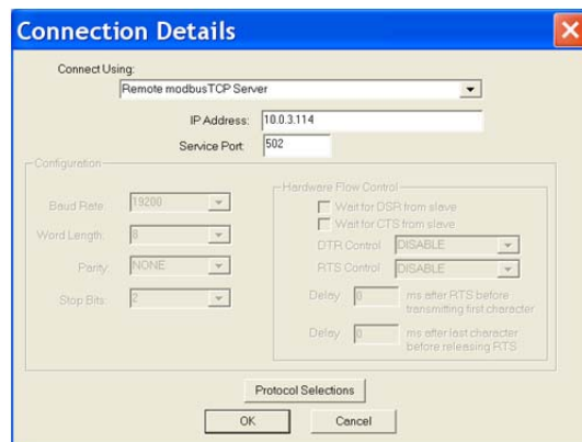
Figure 8.a - Remote connection example
